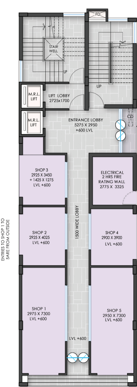
Ground Floor Plan of Block 5
