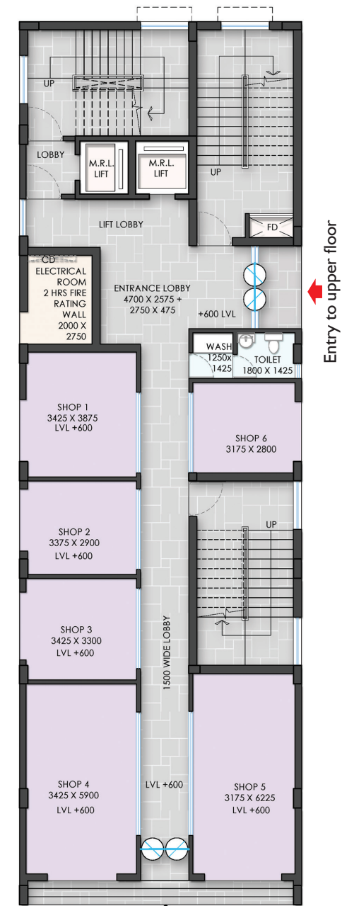
Ground Floor Plan of Block 4
