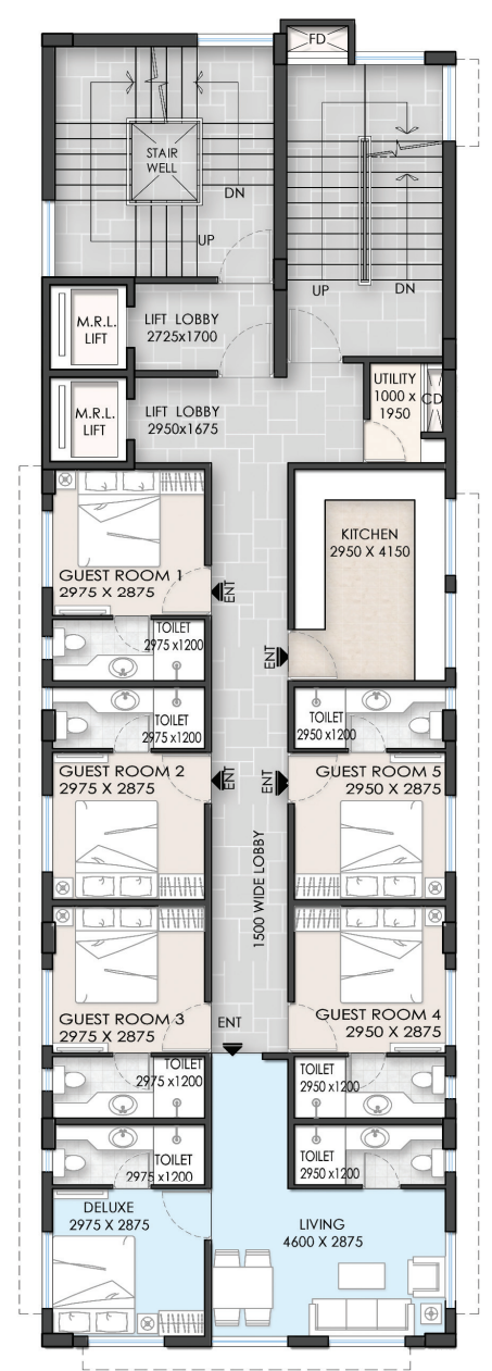
BLOCK 5 (5th FLOOR)
