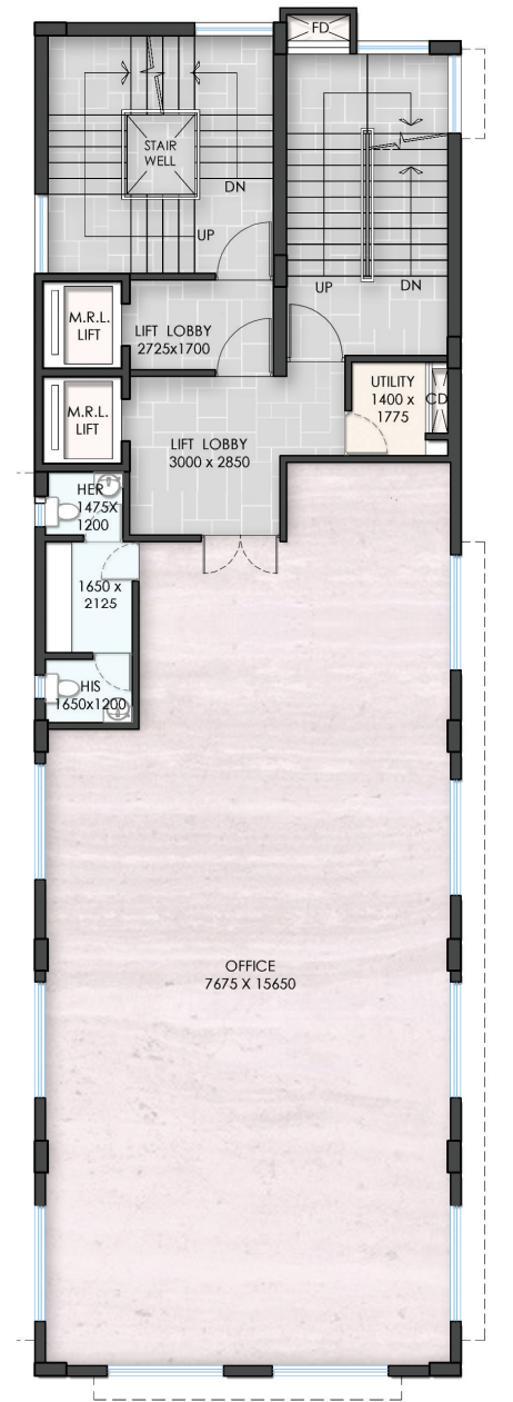
BLOCK 5 (3rd FLOOR)
